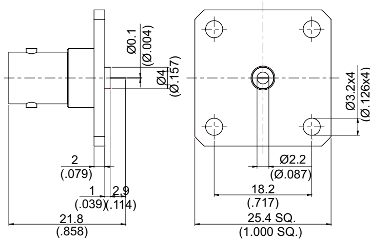
MOUNTING HOLE
