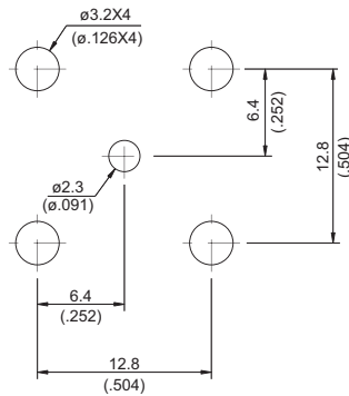
MOUNTING HOLE
